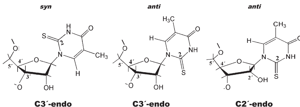
FIGURE 3: Local structural impact of chemically simple modifications. Nucleotide conformations are illustrated with s^2T , a modification typically occurring at position 54 in thermophiles growing above 80 °C: (left) 3'-endo conformation of the ribose and syn conformation of the base, (middle) 3'-endo conformation of the ribose and anti conformation of the base (most favored in s^2T ), and (right) 2'-endo conformation of the ribose and anti conformation of the base.
